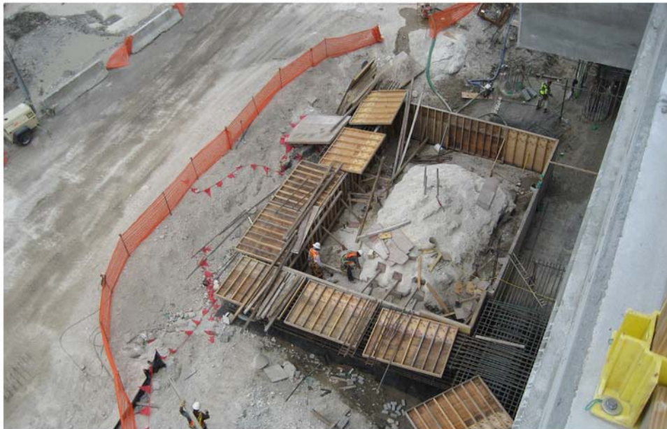
Miami Intermodal Center Construction: Progress Photo March 13, 2009 Rental Car Center (RCC): FM # 249937-5 / MIC-MIA Station: FM # 406800-6 Construction of Stair #4 & #5 for MIC-MIA Station
